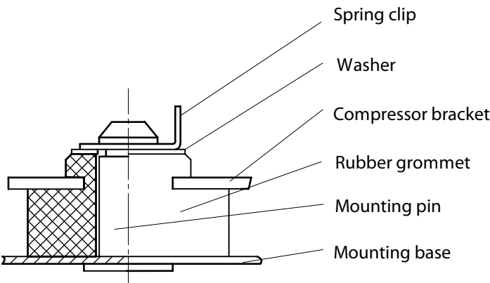
SNAP-ON mounting
