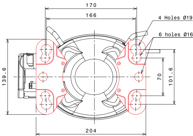
American mounting feet
