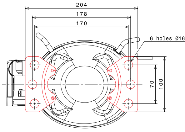
European mounting feet
