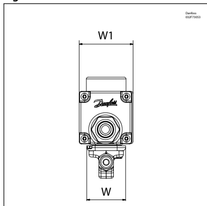
Figure 55: End view
