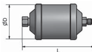
PR Female / Male Flare
