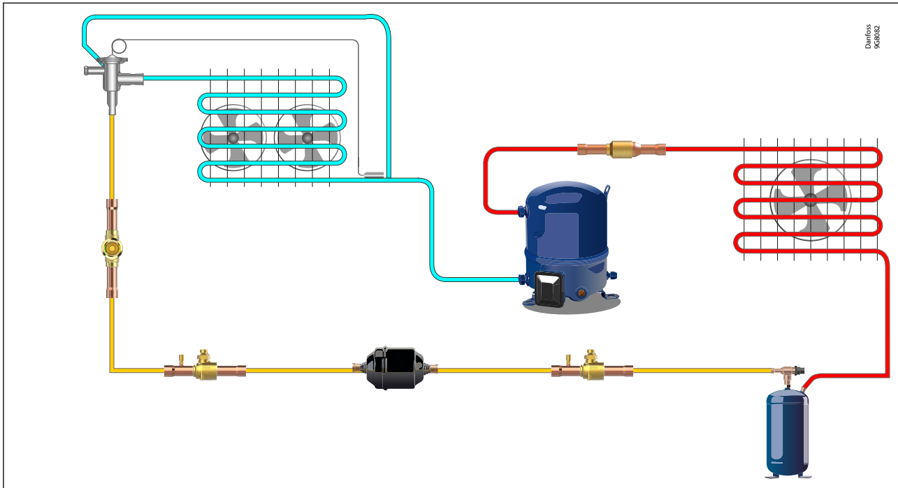
Figure 1: Application Diagram
