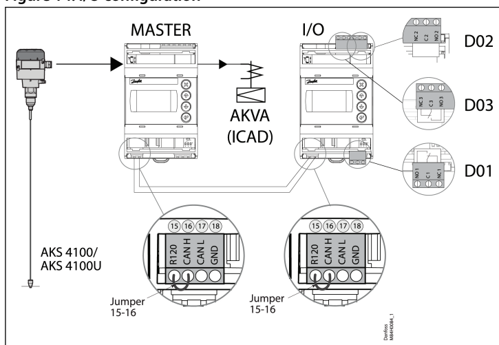
Figure 14: I/O configuration
