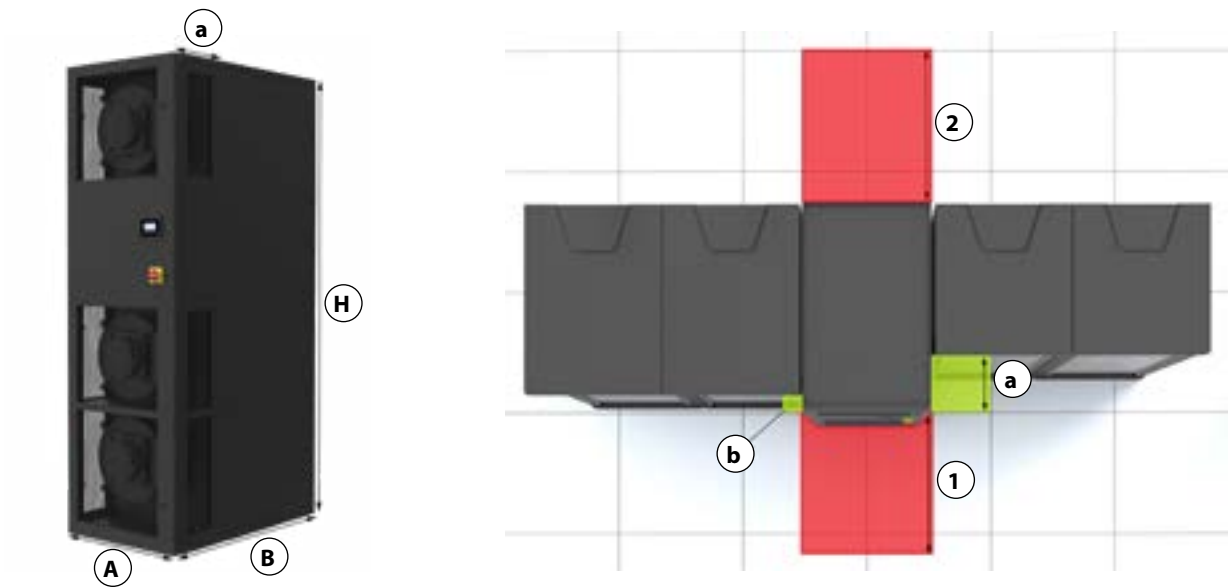
Series R clearance spaces
