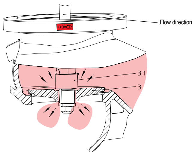
Balancing plug
