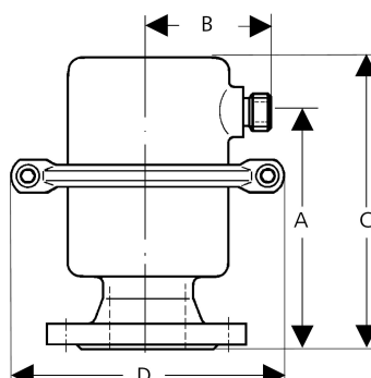
EB 1.12 DN 65 - 100
